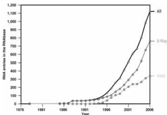
Fig. (1). Yearly growth of RNA structure deposition in the RNABase database. Black curve shows all entries in the RNABase, dark-grey curve shows only entries that were determined by X-Ray experiments and light-grey curve shows those determined by Nuclear Magnetic Resonance experiments.
